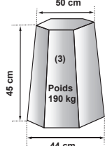
BORNE HEXAGONALE
